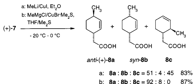
Scheme 4. Regioselectivity in reactions with organocopper compounds
