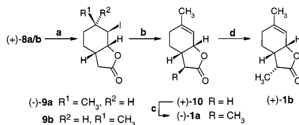
Scheme 5. Reagents and conditions: (a) KI, \text{I}_2 , \text{NaHCO}_3 , \text{H}_2\text{O} /THF, room temp. (95%, dr = 92:8; after recrystallization: 60%, dr > 99:1); (b) DBU, THF, reflux (92%); (c) LDA, MeI, THF, –78 °C (79–90%); (d) LDA, THF, then \text{H}_2\text{C}(\text{COOtBu})_2 , –78 °C (61–74%)
