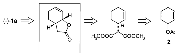
Scheme 1. Retrosynthetic analysis
