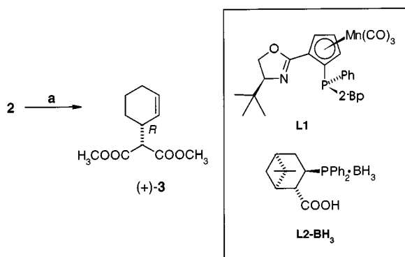
Scheme 2. Reagents and conditions: (a) procedure 1: 0.1 mol-% of [\text{C}_3\text{H}_5\text{PdCl}]_2 , 0.12 mol-% of L1 , THF, \text{NaCH}(\text{COOCH}_3)_2 , 5 °C (88%, 82% ee ); procedure 2: 3.0 mol-% of [\text{C}_3\text{H}_5\text{PdCl}]_2 , 9.0 mol-% of L2 , THF, \text{LiCH}(\text{COOCH}_3)_2 , room temp. (91%, 95% ee )
