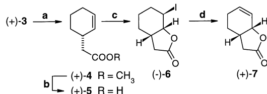
Scheme 3. Reagents and conditions: (a) NaCl, \text{H}_2\text{O} , DMSO, 160 °C (74%); (b) NaOH, 120 °C (95%); (c) KI, \text{I}_2 , \text{NaHCO}_3 , \text{H}_2\text{O} (82%, > 99.9% ee ); (d) DBU, THF, reflux (82–91%)
